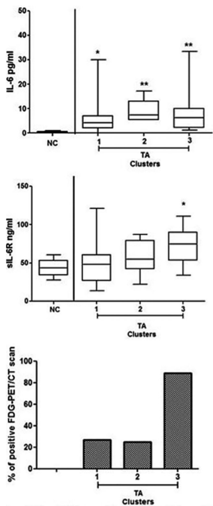
Supplementary Fig. S1. IL-6 and sIL-6R circulating levels in three TA groups identified by cluster analysis.
