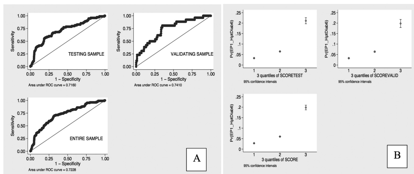
Supplementary Figure 1. Validation of the discrimination ability of the predictive model.
