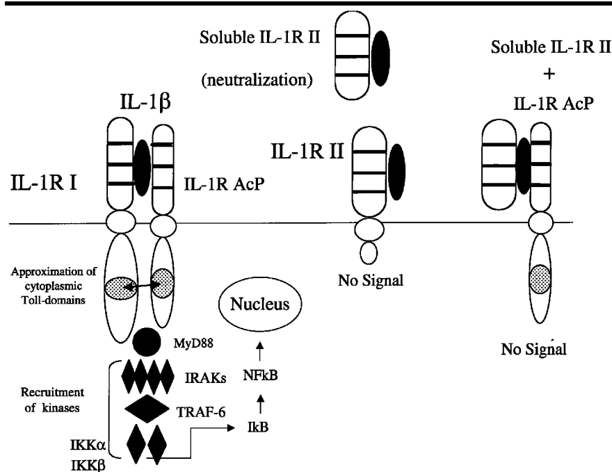
Fig. 1. IL-1 signal transduction. The IL-1RI binds IL-1b and this complex recruits the IL-1R AcP to form a ternary complex. As a result, the Toll-domains present in the cytoplasmic segments of both receptor chains approximate and this results in the binding of MyD88 to the complex. There are four kinases termed IL-1 receptor activating kinases (IRAK) which are phosphorylated by the IL-1R complex. Another kinase that is phosphorylated in the TNF receptor activating factor-6 (TRAF-6). Following phosphorylation of TRAF-6, two additional kinases are phosphorylated: inhibitory- \kappa B (I \kappa B) kinase- \alpha and I \kappa B kinase- \beta (IKK \alpha , IKK \beta ). These latter kinases, in turn, phosphorylate I \kappa B itself resulting in proteolysis of I \kappa B and the release of NF \kappa B. NF \kappa B translocates to the nucleus and acts to trigger gene expression. When IL-1b binds to the cell-surface IL-1R type II (IL-1RII), there is no signal transduction since this receptor (decoy receptor) lacks a cytoplasmic domain. Soluble IL-1RII also can bind IL-1b and this results in neutralization of IL-1b. In addition, the soluble IL-1RII-IL-1b complex may bind to the IL-1R AcP and this complex does not signal but rather deprives the IL-1RI of the IL-1R AcP to form an active complex.
