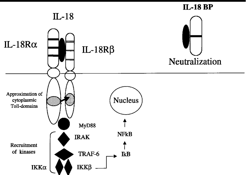
Fig. 2. IL-18 signal transduction. The IL-18Ra chain binds IL-18 and this complex recruits the IL-18Rb chain to form a ternary complex. As a result, the Toll-domains present in the cytoplasmic segments of both receptor chains approximate and this results in the binding of MyD88 to the complex. There are four kinases termed IL-1 receptor activating kinases (IRAK) which are phosphorylated by the IL-1R complex. It is unclear which of these are activated by IL-18. Similar to IL-1, the TNF receptor activating factor-6 (TRAF-6) is phosphorylated. Following phosphorylation of TRAF-6, two additional kinases are phosphorylated: inhibitory- \kappa B (I \kappa B) kinase- \alpha and I \kappa B kinase- \beta (IKK). These latter kinases, in turn, phosphorylate I \kappa B itself resulting in proteolysis of I \kappa B and the release of NF \kappa B. NF \kappa B translocates to the nucleus and acts to trigger gene expression. When IL-18 binds to the IL-18BP, this results in neutralization of IL-18.
